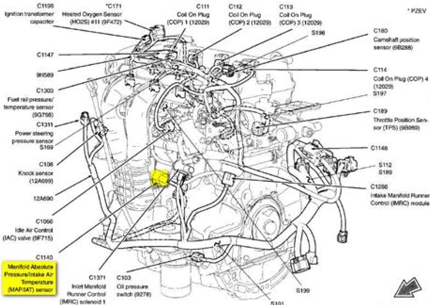
engine, front - 2.0L
