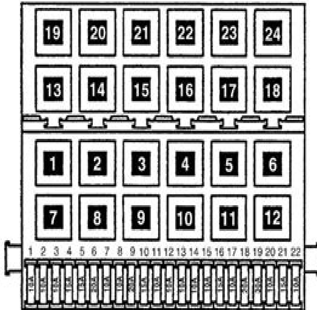
Fuse/Relay Panel
