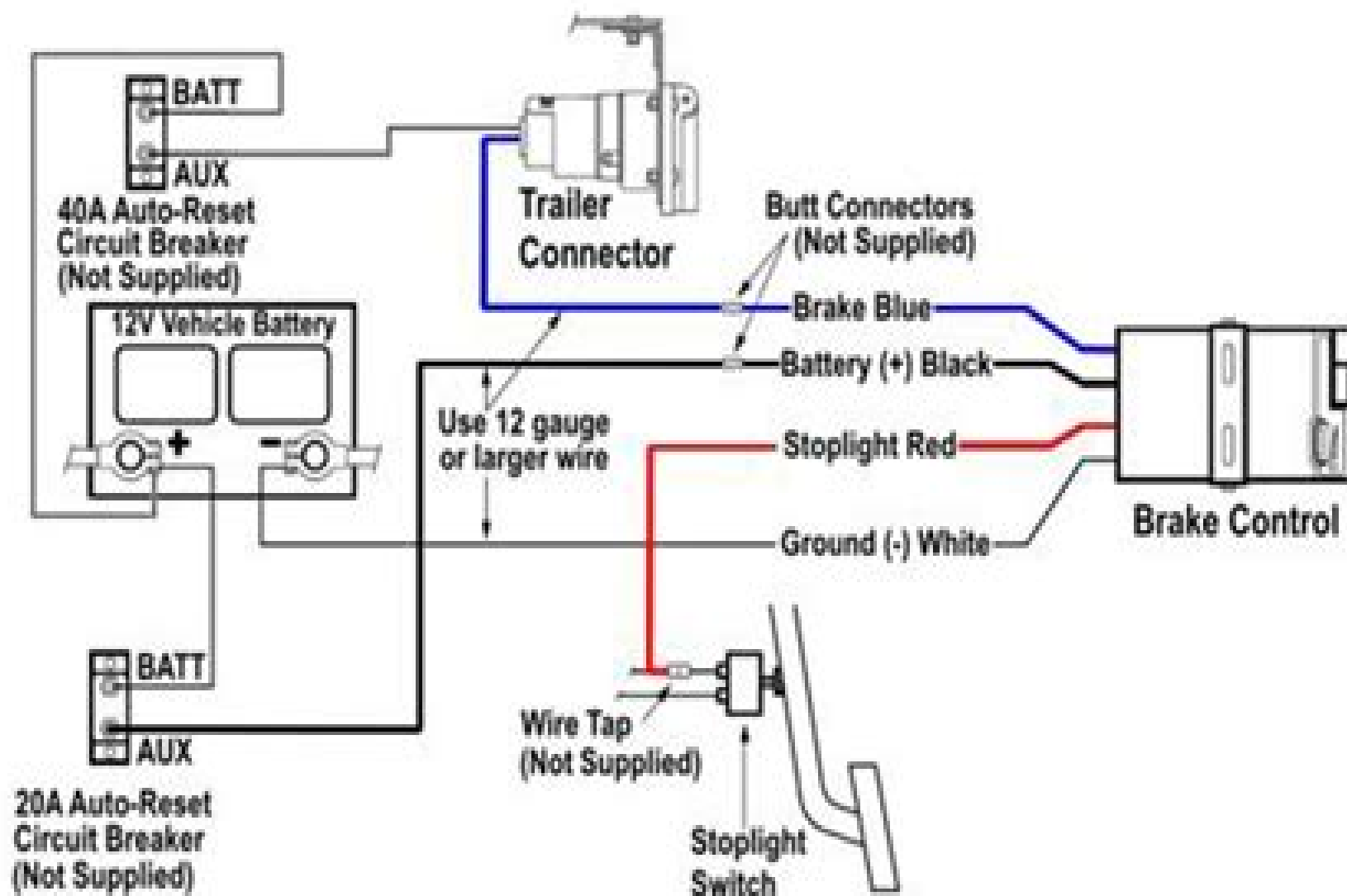
Brake Controller Wiring Diagram
