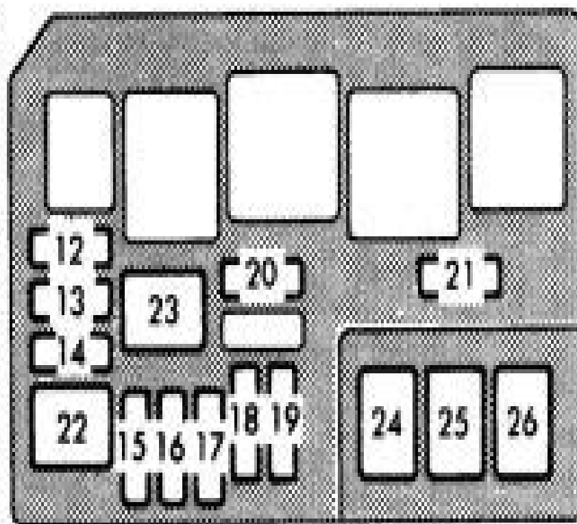
ENGINE COMPARTMENT
