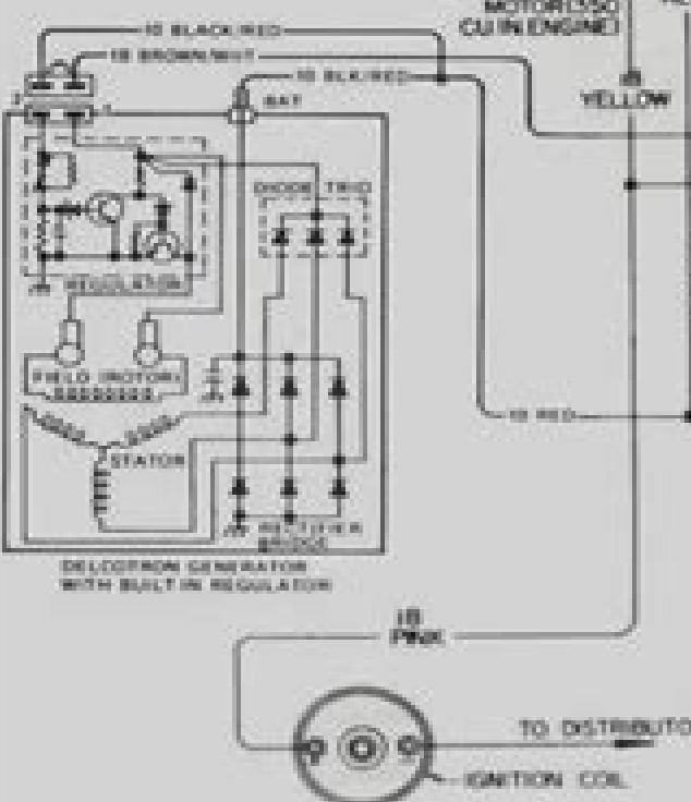
PART OF ENGINE WIRING HARNESS
