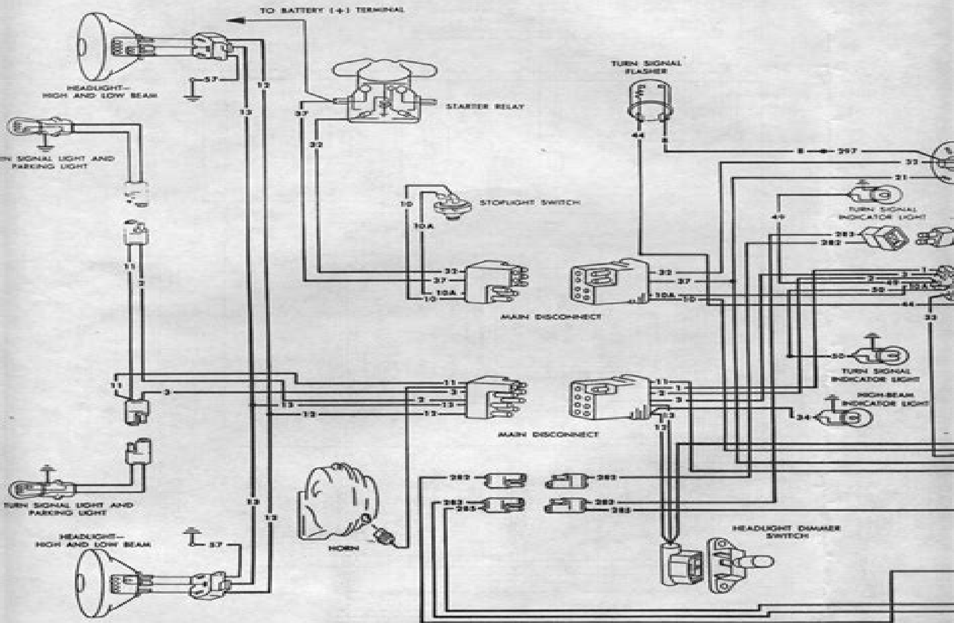
1966 BRONCO EXTERIOR LIGHTING, TUR
