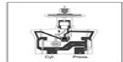
Figure 13B: Normally Closed, Operator Pressurized
