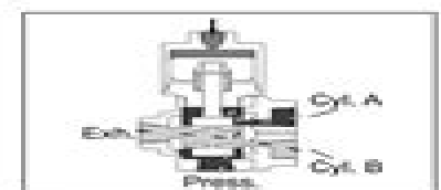
Figure 14B: Operator Pressurized
