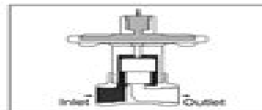
Figure 11B: Normally Open, Operator Pressurized
