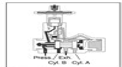
Figure 14D: Operator Pressurized
