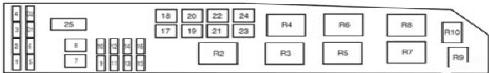
Assignment of the fuses in the Power distribution box (2005)
