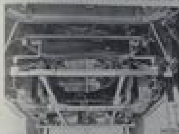
Fig. 14-Frame Alignment Clamping Bars in Position
