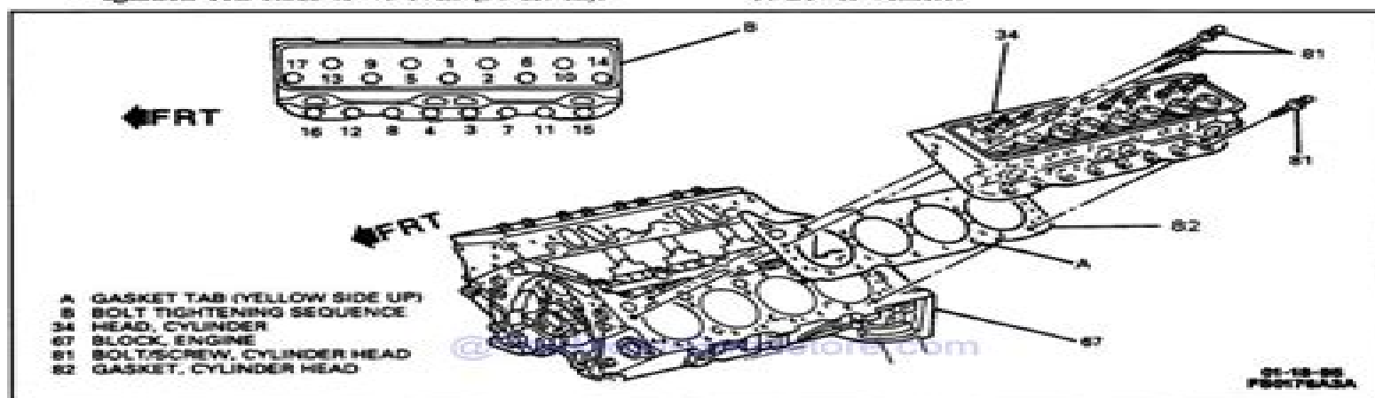
Figure 20 - Cylinder Head
