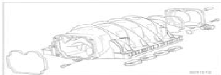
Fig. 49. Crankcase ventilation pressure regulating valve cover at rear of intake manifold (arrows).
