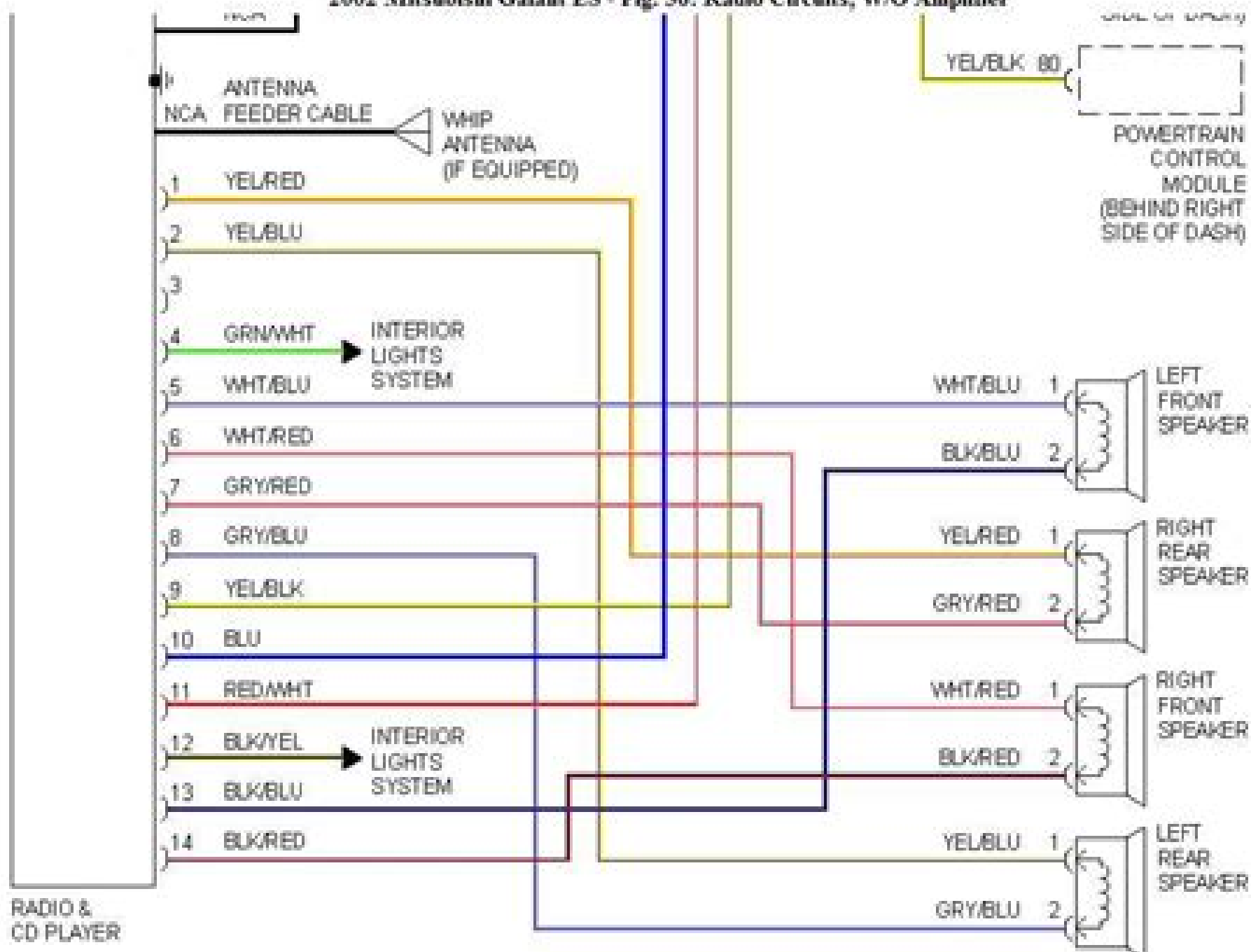
2002 Mitsubishi Galant ES - Fig. 36: Radio Circuits, W/O Amplifier
