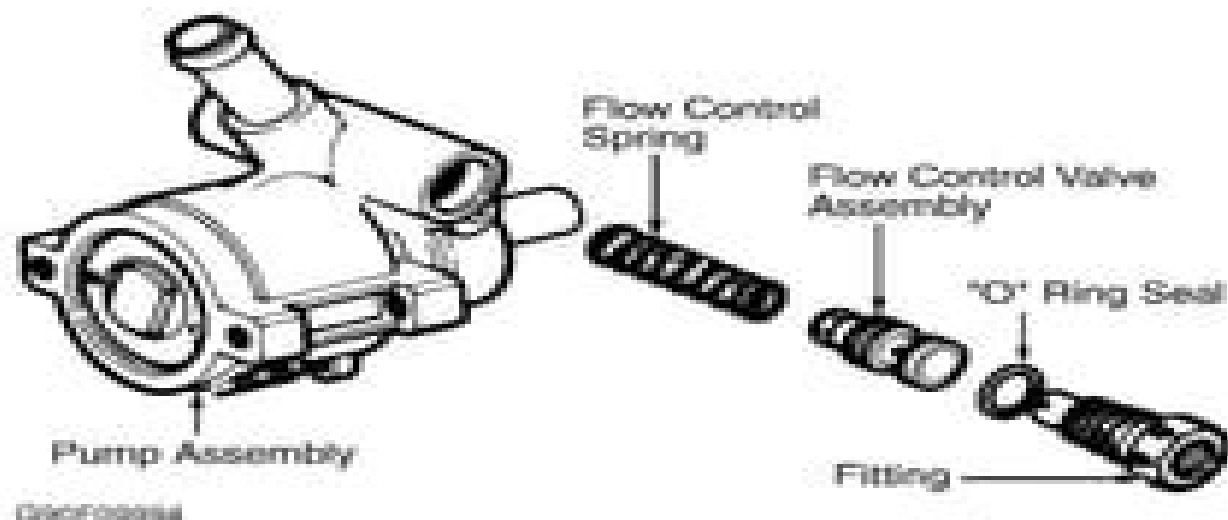
Fig. 4: Exploded View Of Flow Control Valve Assembly (Typical) Courtesy of GENERAL MOTORS CORP.
