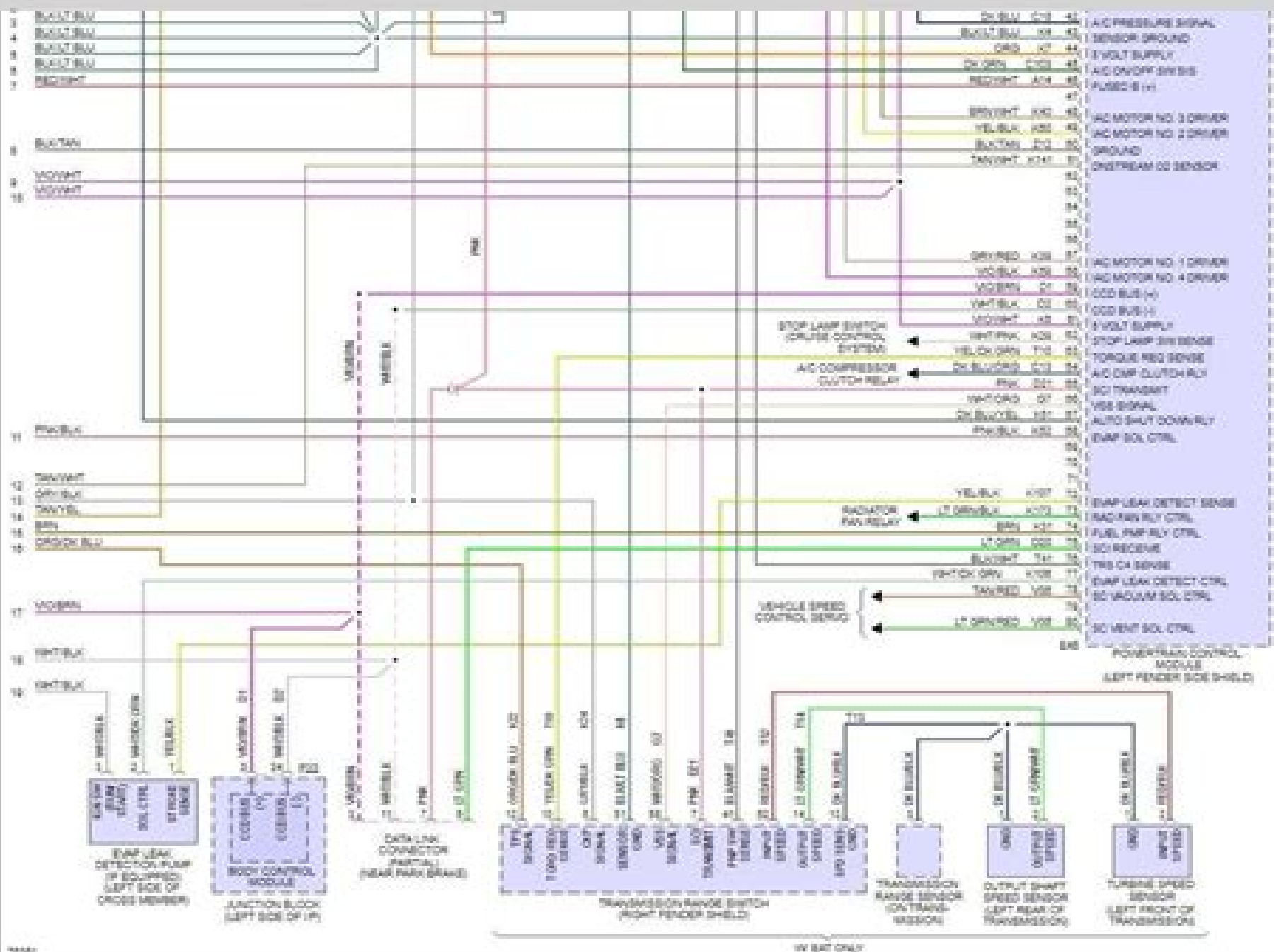
Fig 6-33L Engine Performance Circuits (3 of 3)
