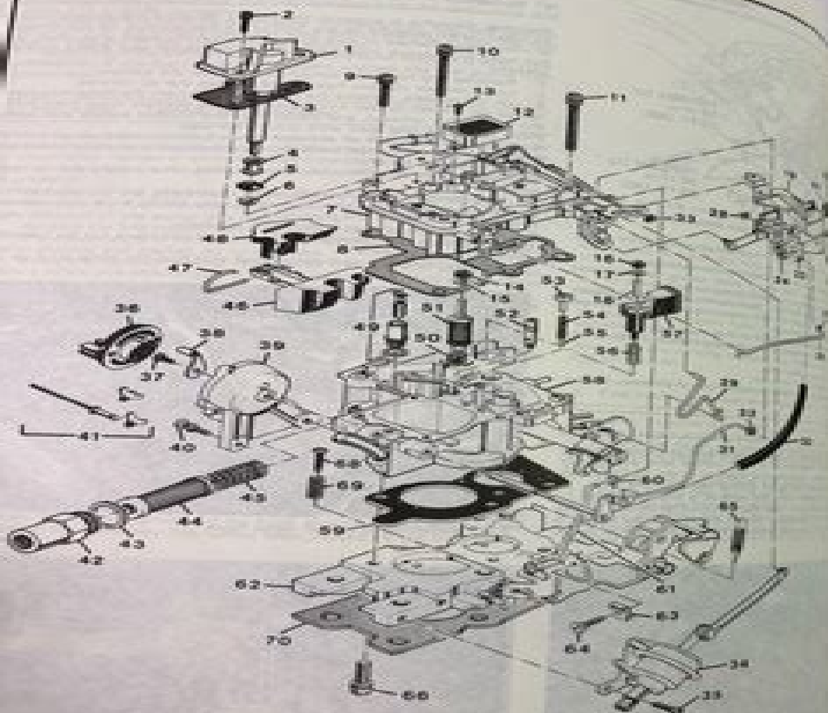
Fig. 4.3 B25E carburetor - exploded view (Sec 8)
