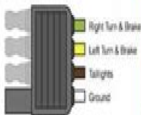
4 Wire Flat
