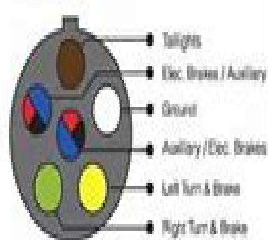
6 Pole Round
