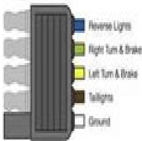
5 Wire Flat
