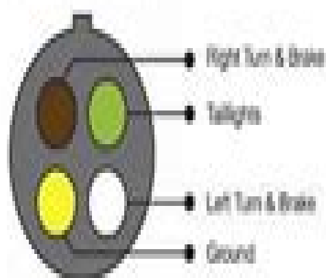
4 Pole Round
