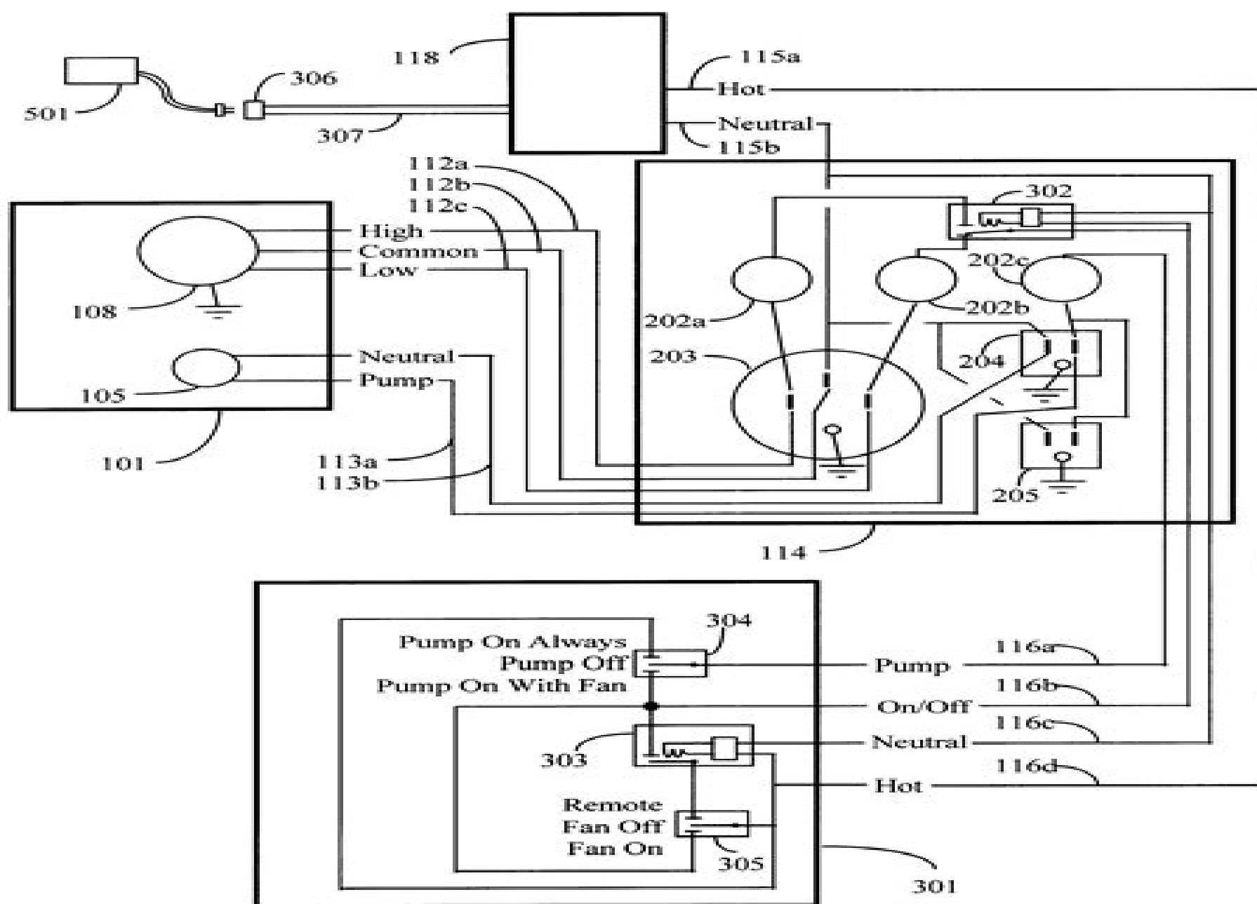
EVAPORATIVE COOLER WIRING SCHEMATIC IN ACCORDANCE WITH INVENTION
