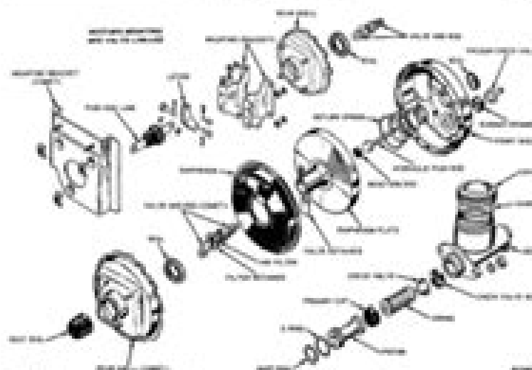
FIG. 41—Front Brake Disassembly
