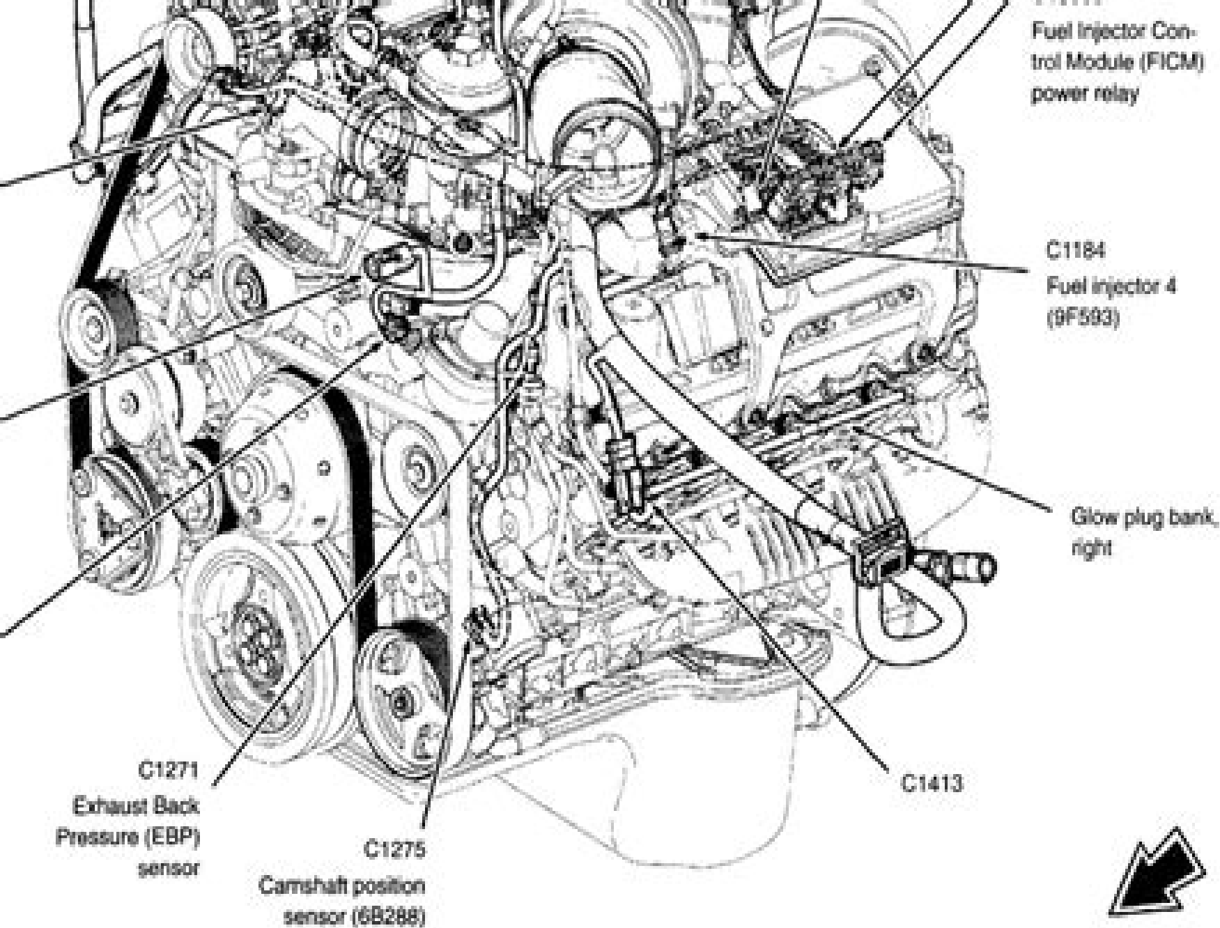
6.0L Diesel engine, LH side
