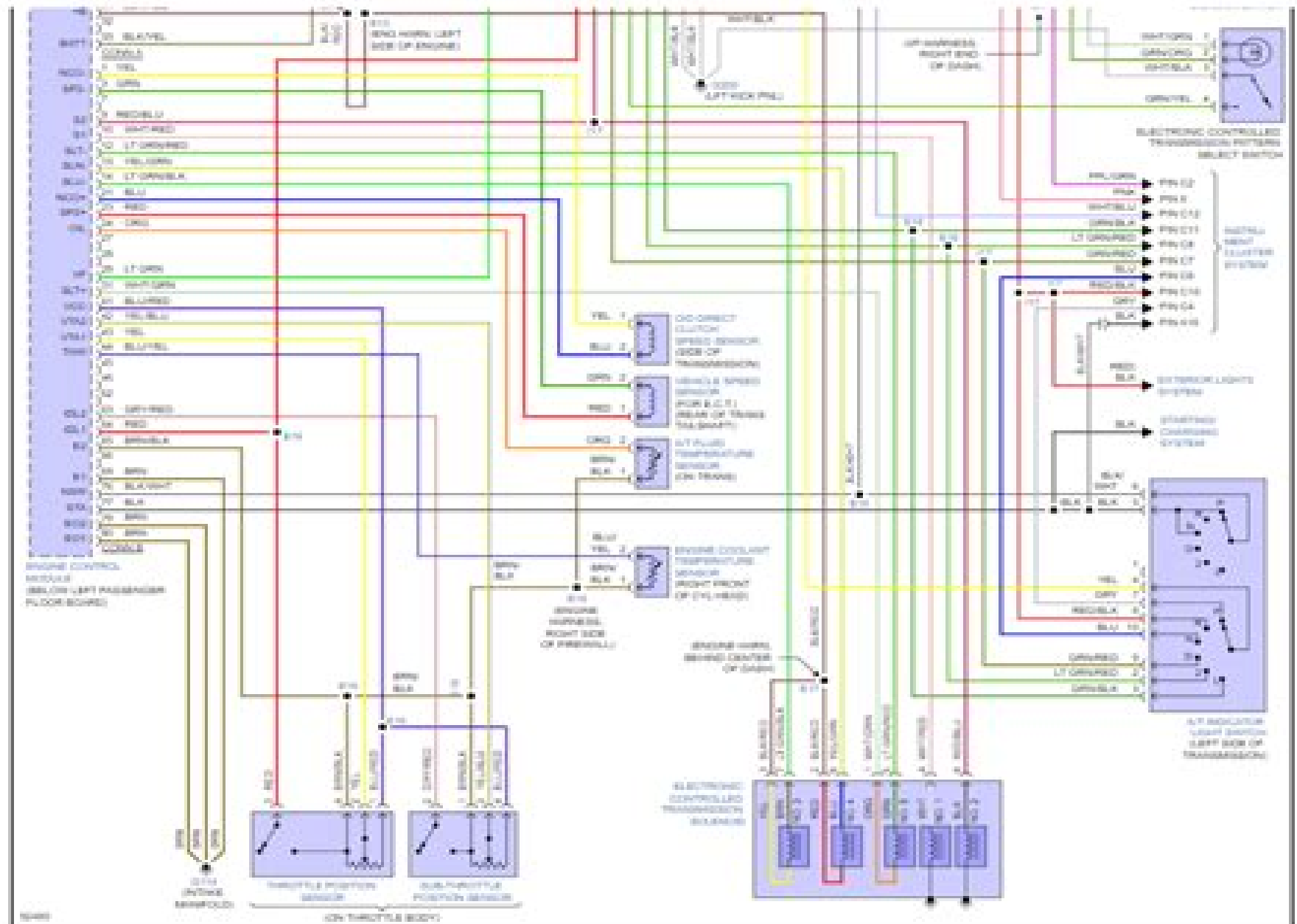
Fig 2: 3.0L Turbo, Transmission Circuit
