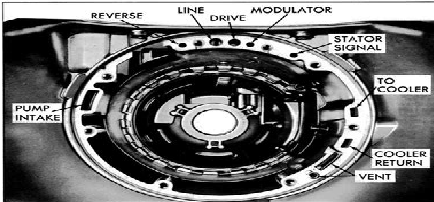
Fig. 7-20 Transmission Case Oil Passages - Front View
