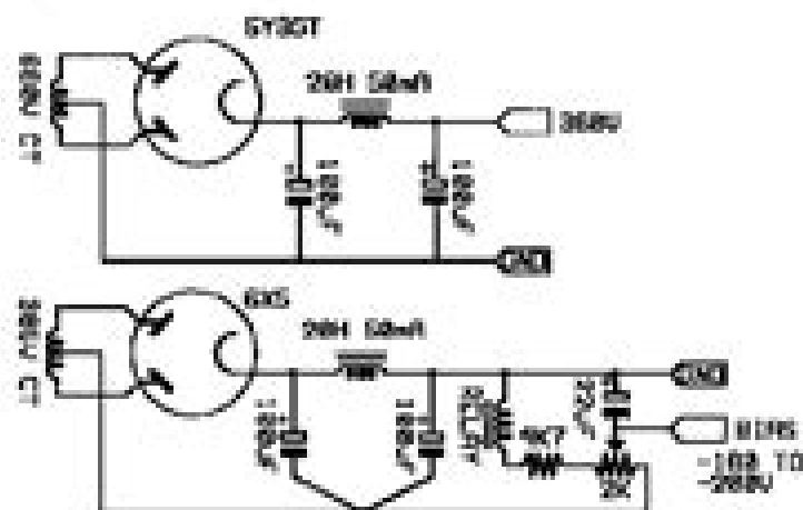
6AR5, 2AR5 &amp; 7044 HT SUPPLY
