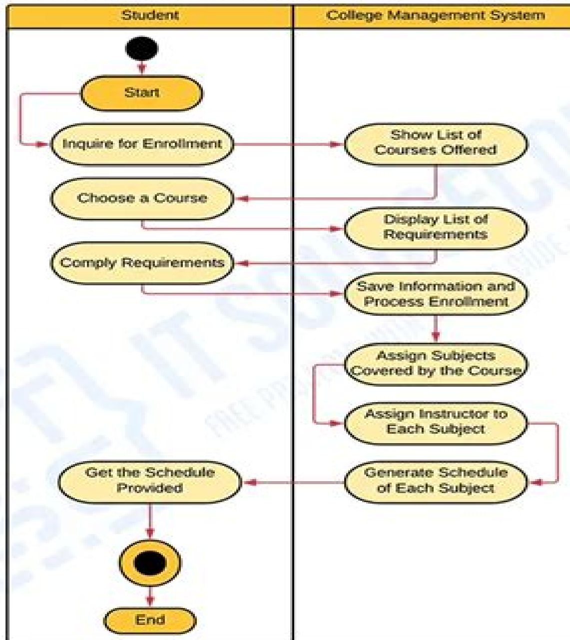
ACTIVITY DIAGRAM
