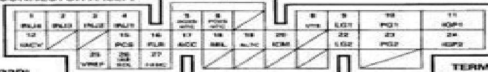
ECM CONNECTOR A (32P)
