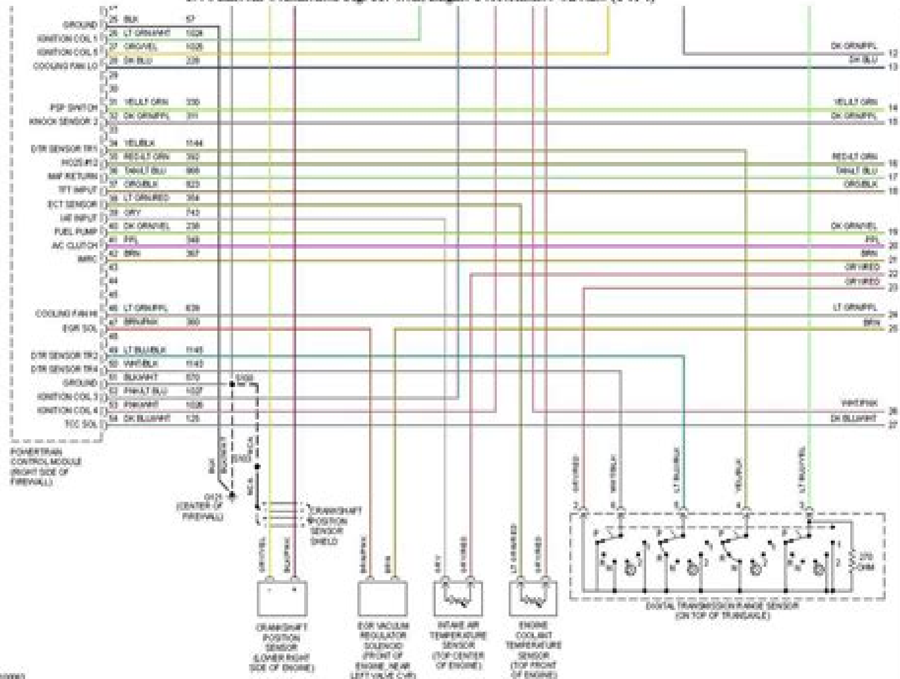
1998 Lincoln Continental-Pg. 11: 4.4L Engine Performance Circuits (1 of 4)
