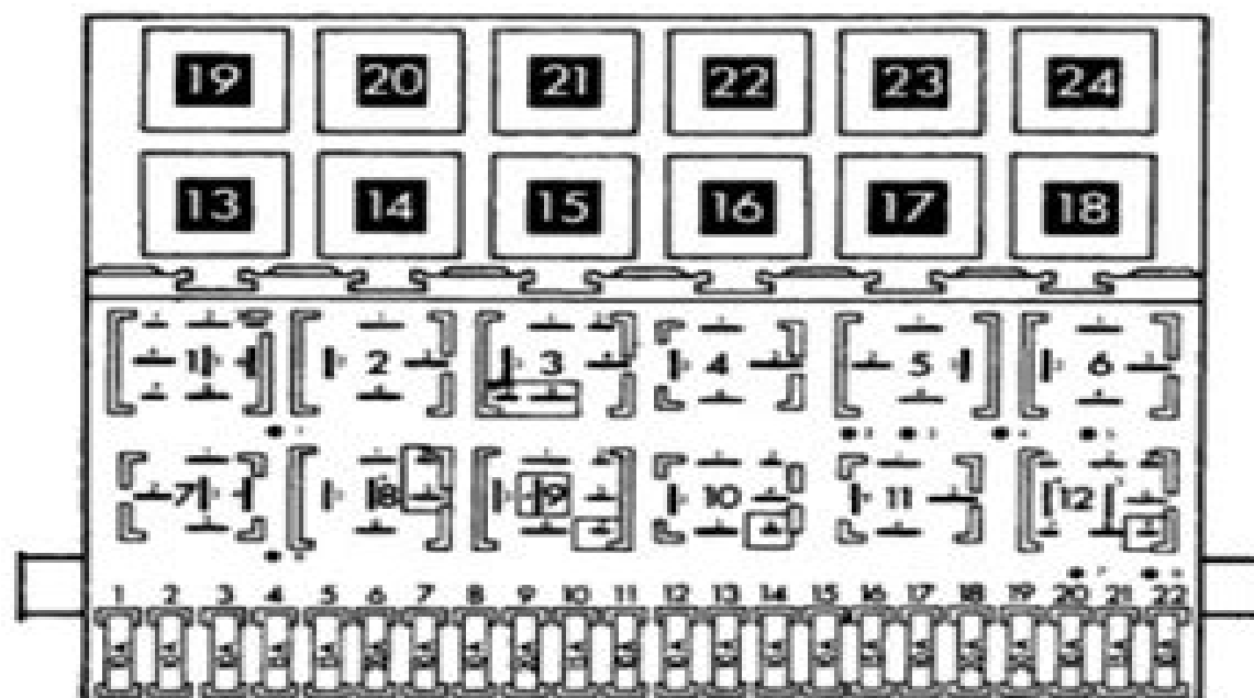
Fig 5: Identifying Underdash Fuse & Relay Panel Components For Golf, GTI & Jetta (1990-96) & Cabrio (1995-96)
