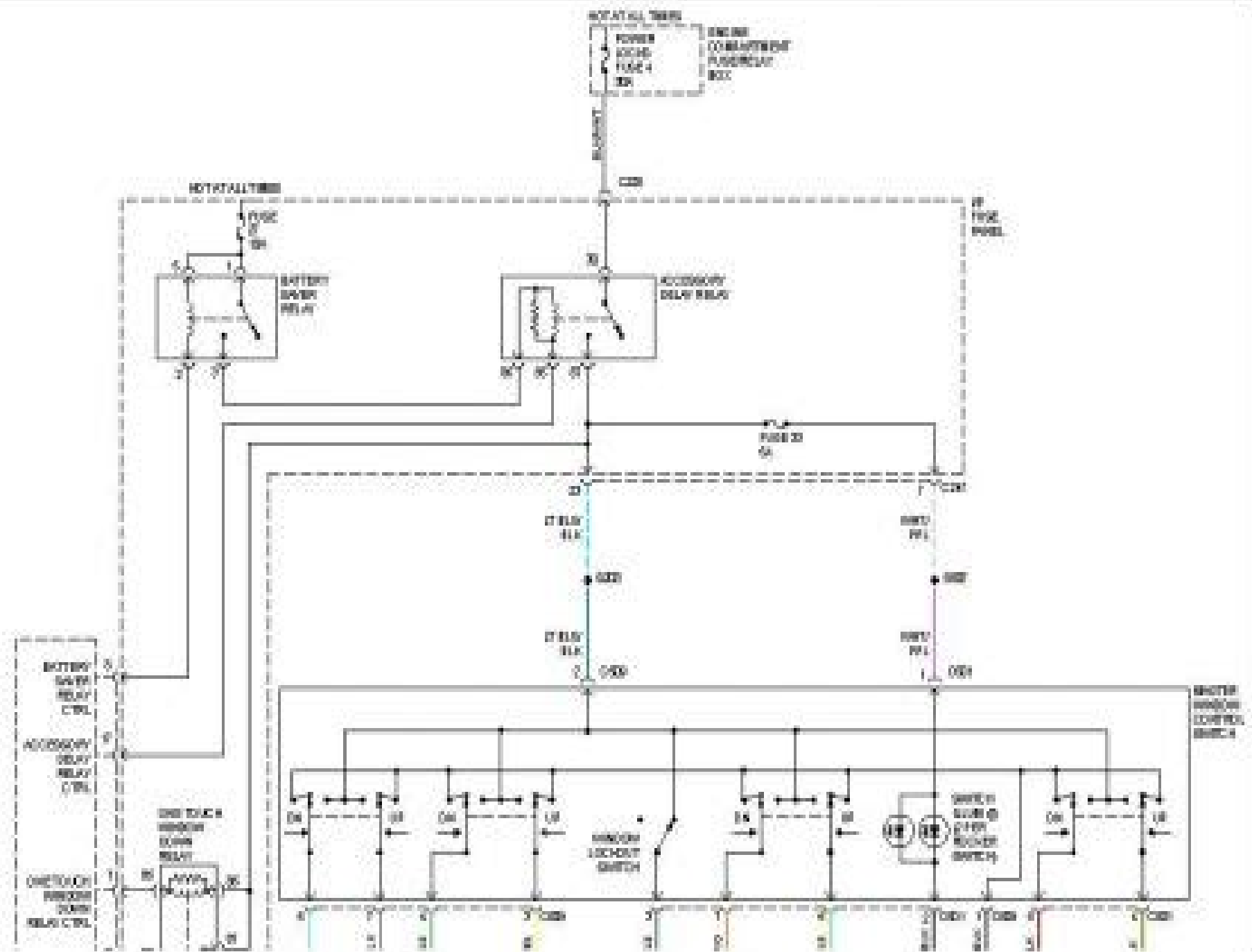
199 Fordaurus LX Reg. 50 Power Window Circuit
