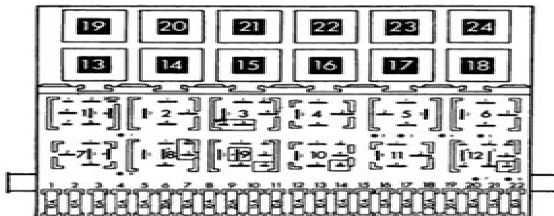
Fig 5: Identifying Underdash Fuse & Relay Panel Components For Golf, GTI & Jetta (1990-96) & Cabrio (1995-96)
