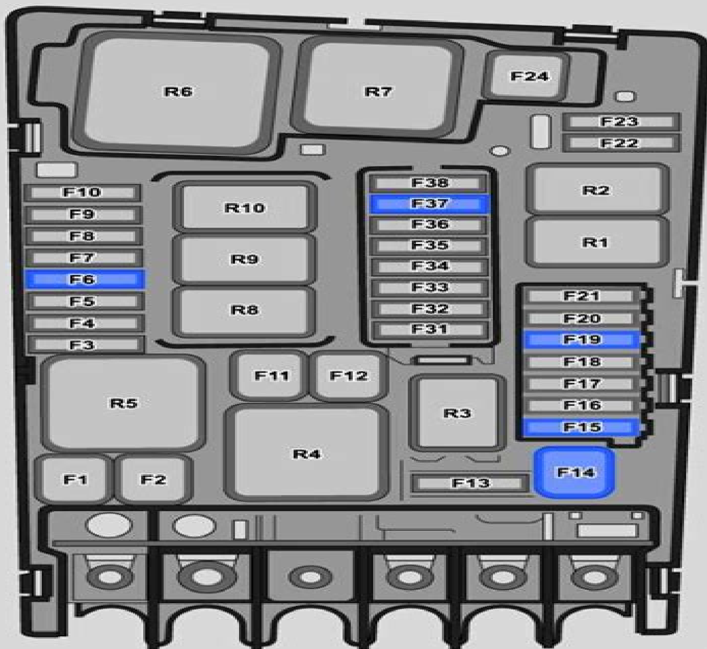
Fig. 1 In the engine compartment: fuse locations.
