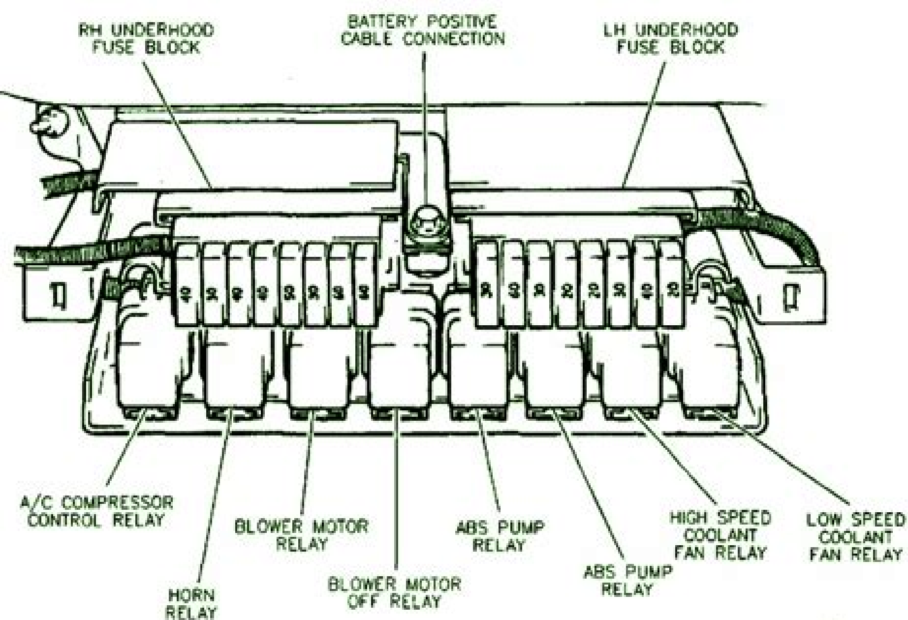
Rear Of Engine Compartment, LH And RH Underhood Fuse Blocks
