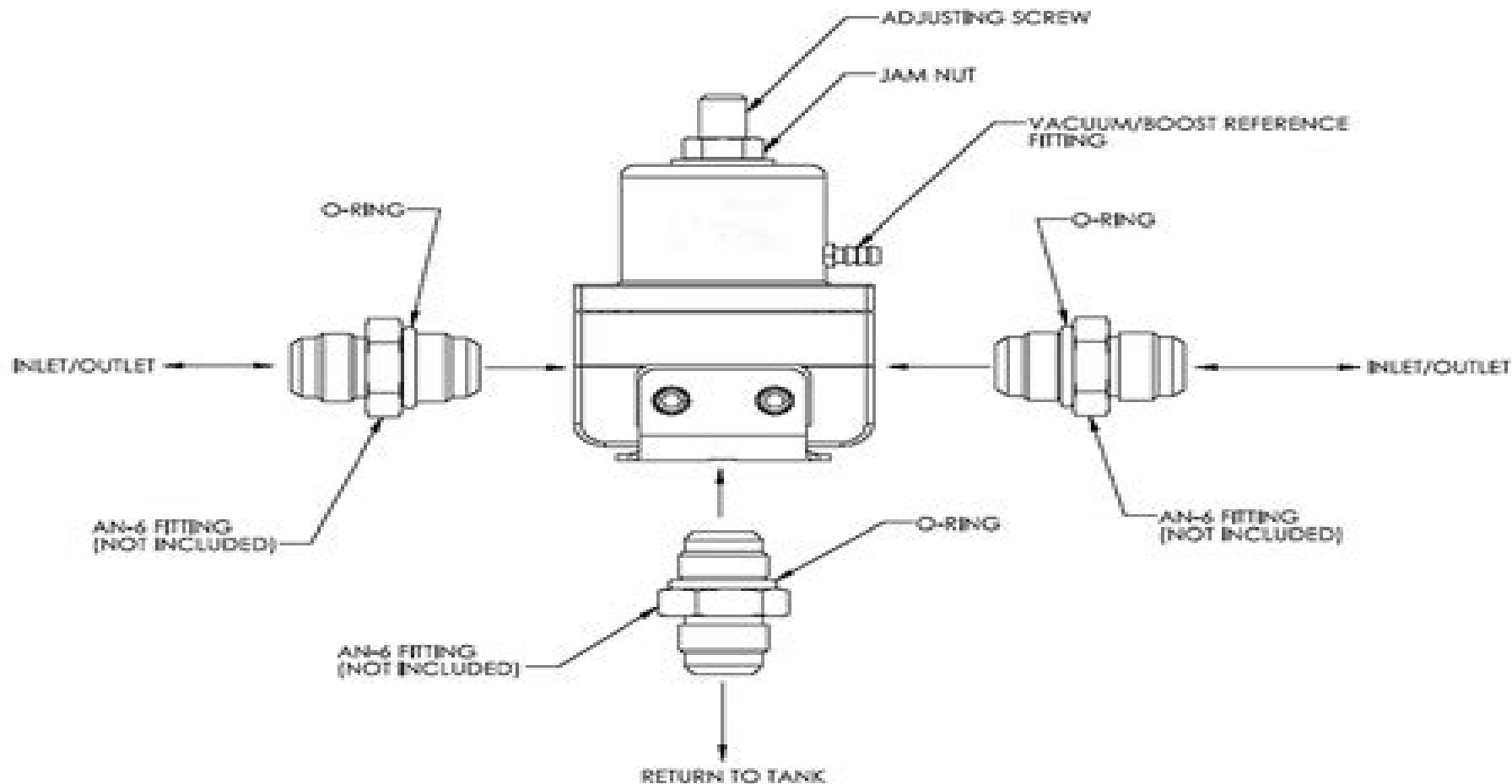
Fuel Pressure Regulator
