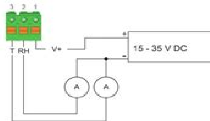
Connection scheme
