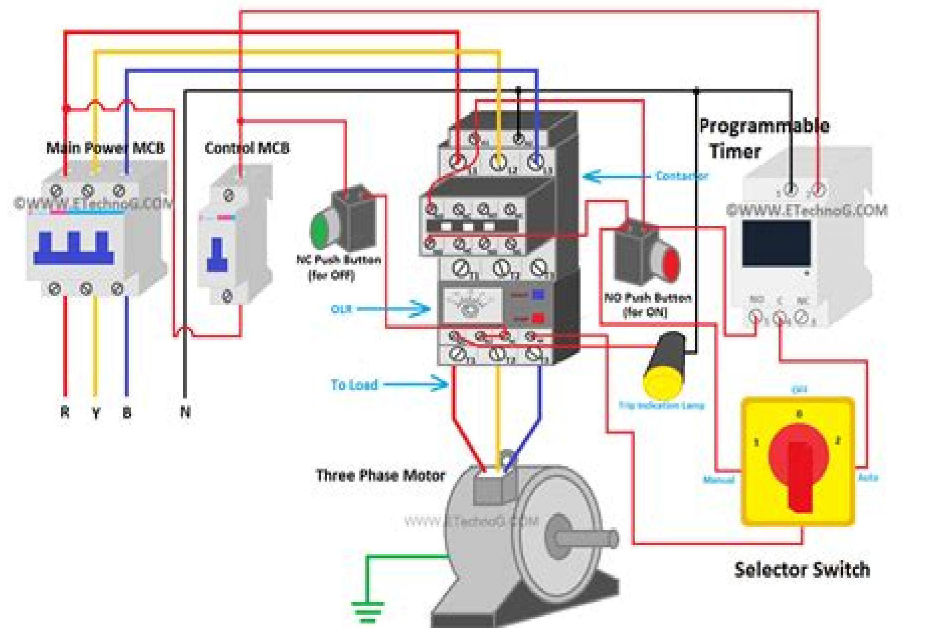
Figure.01: DOL Starter, Motor, and Timer Connection for Auto and Manual Operation
