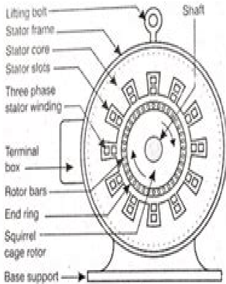
Sectional view
