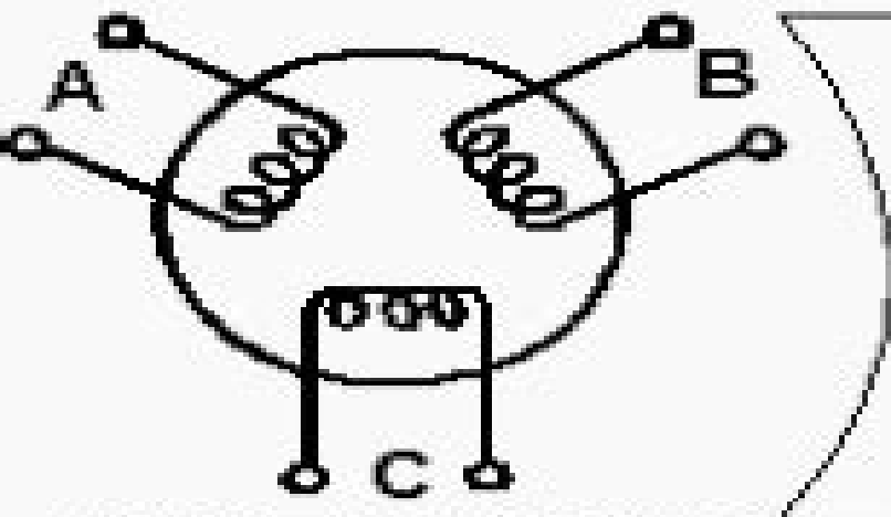
THREE-PHASE ALTERNATOR A
