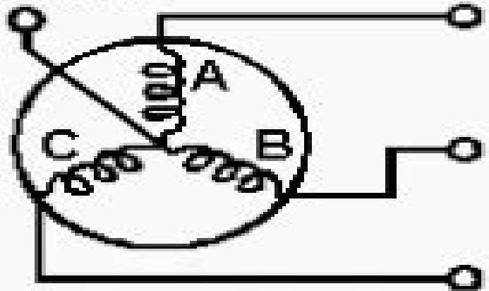
THREE-PHASE WYE CONNECTED B
