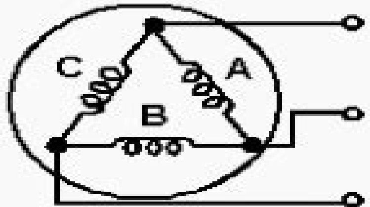
THREE-PHASE DELTA CONNECTED C
