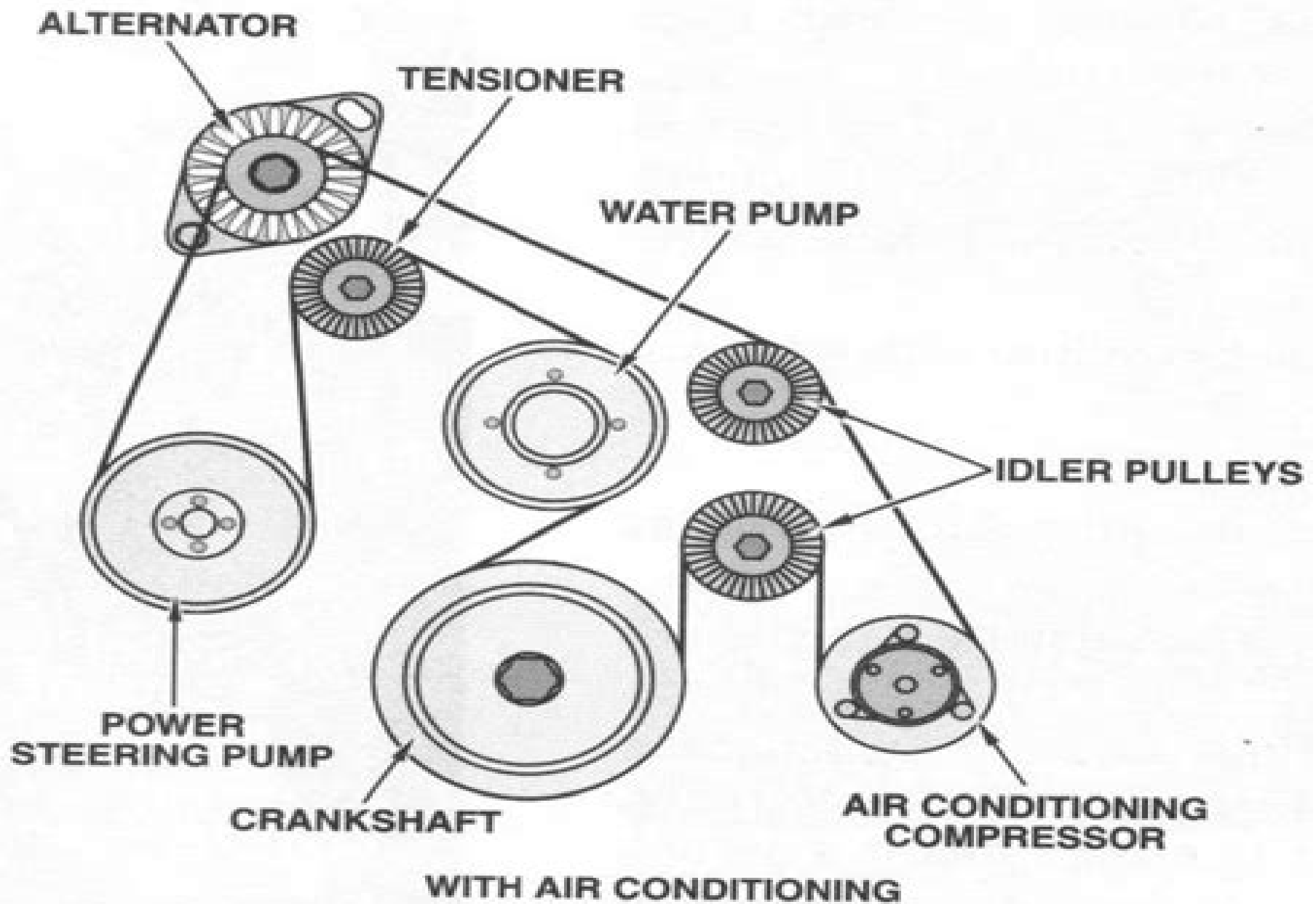
Drive belt installation schematics.
