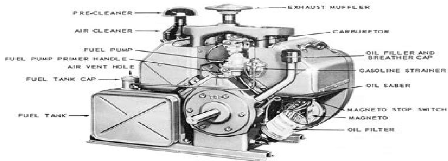
TAKE-OFF (Side Mount Tank) VIEW OF ENGINE
