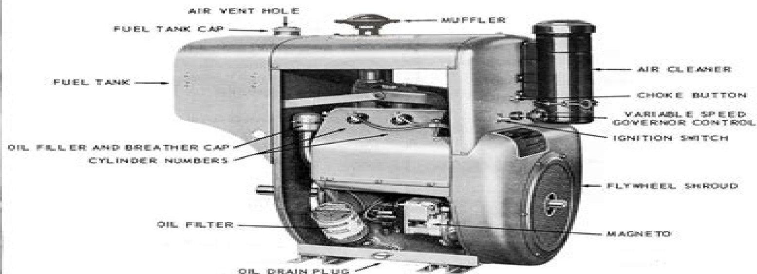
POWER UNIT FAN END VIEW OF ENGINE
