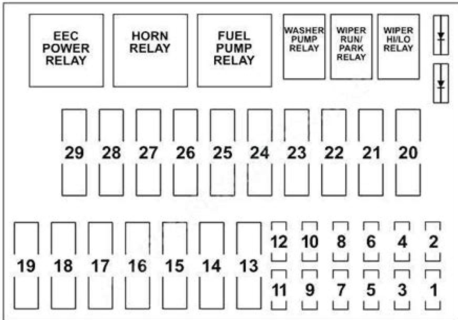
UNDER-HOOD FUSE/RELAY BOX 1997-1998 FORD F150, F250 AND EXPEDITION
