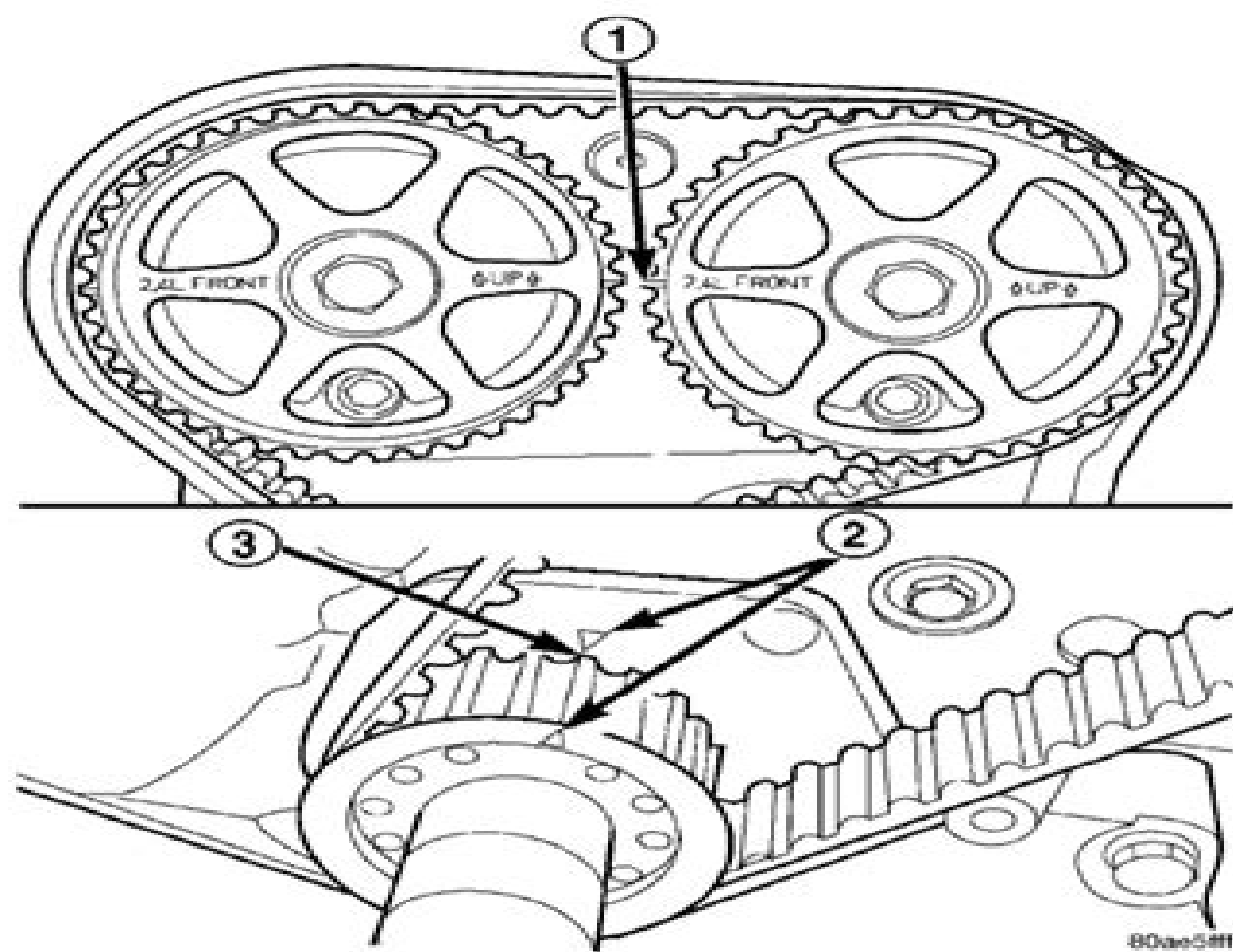
Fig. 122 Crankshaft and Camshaft Timing
