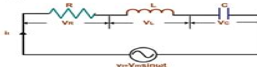
Figure 2.34 Circuit Diagram of Series RLC Circuit
