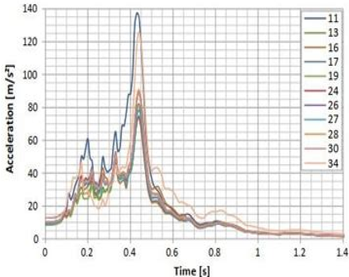
Fig. 63 Case D-1. Horizontal acceleration response spectra at the dam crest (Point C). Results are from Contributors using free-field BCs
