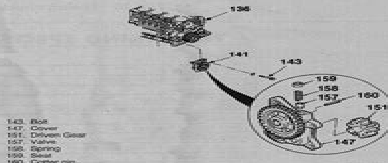
Fig. 24 Oil pump components
