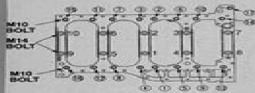
Fig. 20 Crankcase bolt tightening sequence
