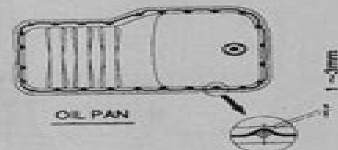
Fig. 22 Oil pan liquid gasket location
