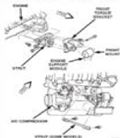
Fig. 22 Engine Mounting—Front 2.0 and 2.4
