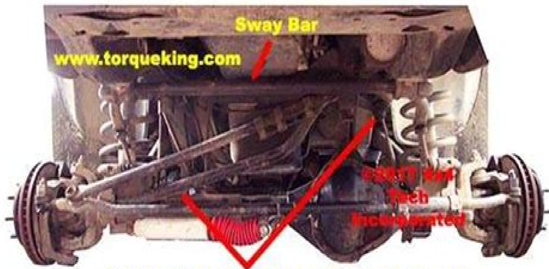
1994-2013 Dodge Ram Coil-5 Link Front Suspension Track Bar Location Dana Axle Shown, AAM Similar
