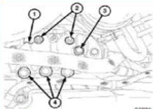
Fig. 96: Power Steering Hose Hold Down, Right Engine Mount Bracket Courtesy of CHRYSLER LLC
