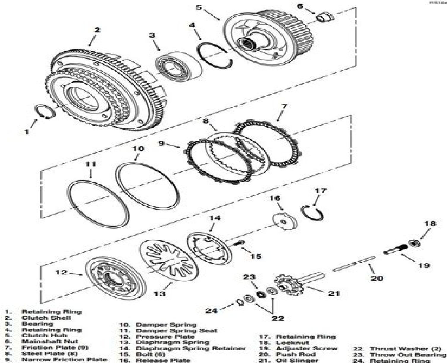
Figure 6-5. Clutch Assembly
