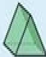
Triangular prism
