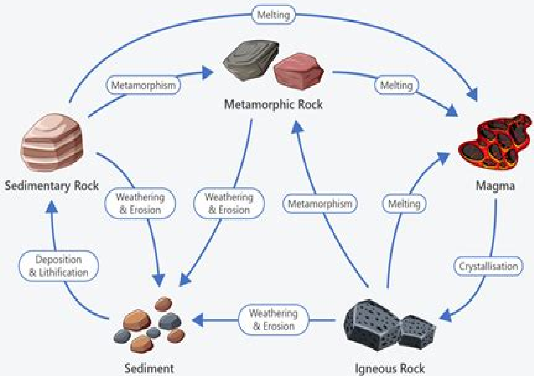
The Rock Cycle
